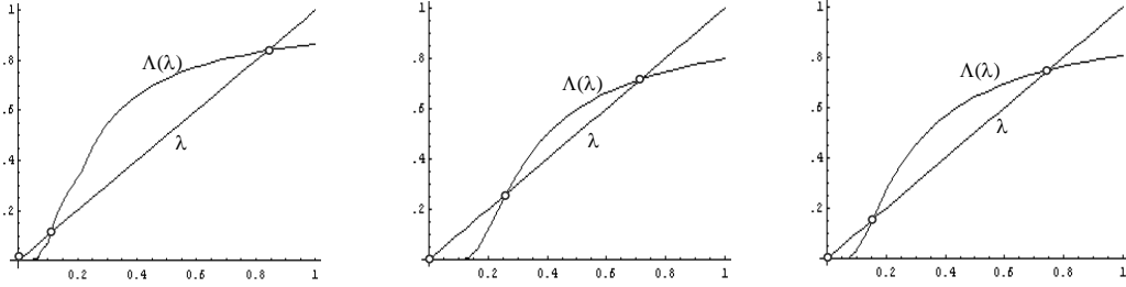
Figure 6.1: Illustrates the fixed points of \Lambda(\lambda) for three numerical examples. The circled points correspond to the neighbor adoption probabilities that determine each Bayes-Nash equilibrium. In the first figure, n = 10, r = 0.1, c = 0.2 and F(\theta) = \theta . In the second figure, n = 100, r = 0.1, c = 2 and F(\theta) = \theta . In the final figure, n = 100, r = 0.1, c = 1 and F(\theta) = 1 - (1 - \theta)^2 . In each of the figures (though not clearly visible), \Lambda(\lambda) has a portion between 0 and a positive value where \Lambda(\lambda) = 0 .
